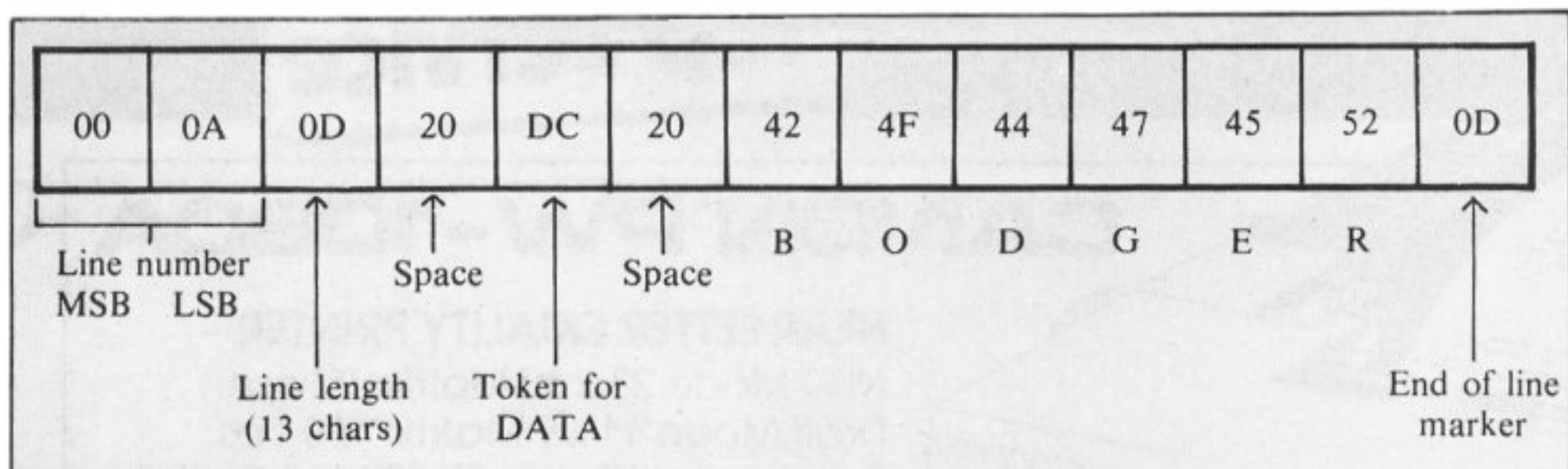
Figure II: A Basic line in practice: 10 DATA BODGER
