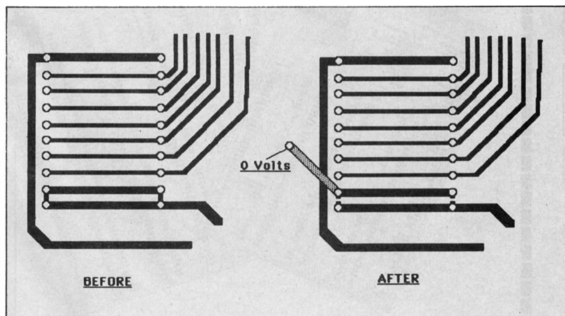
Figure IV: Keyboard modification
