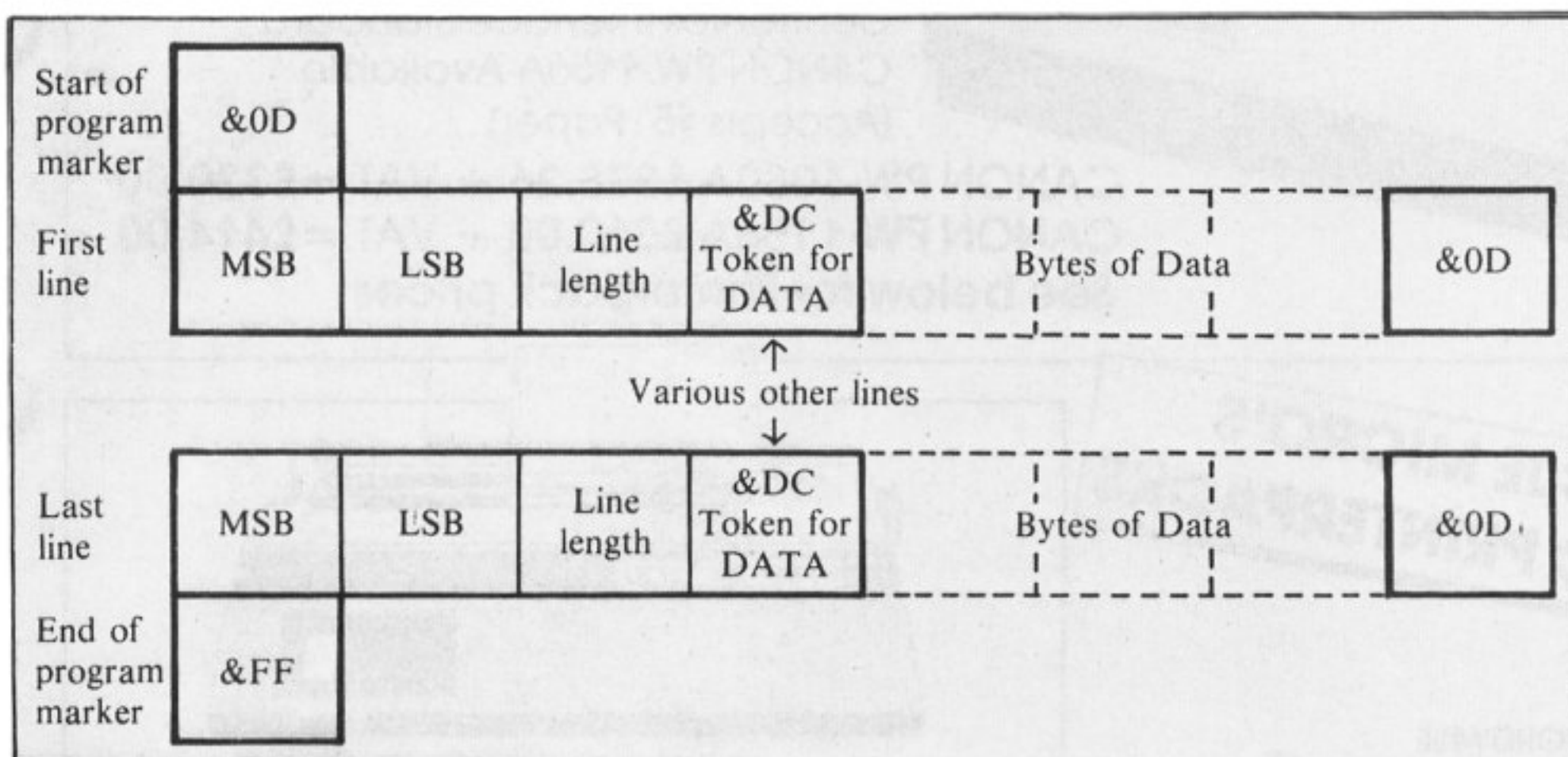
Figure III: Structure of program created by Data Maker
