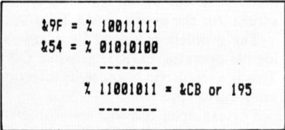
Diagram IV: EORing two bytes
