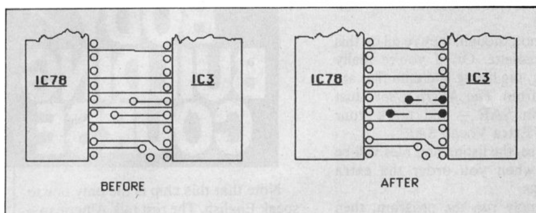
Figure III: Breaking wrong connection
