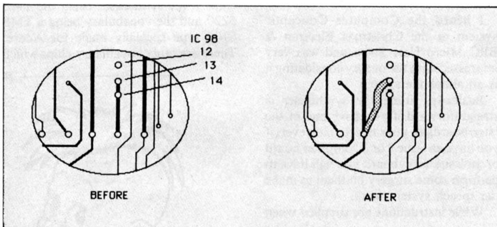
Figure I: IC98 cut track and link
