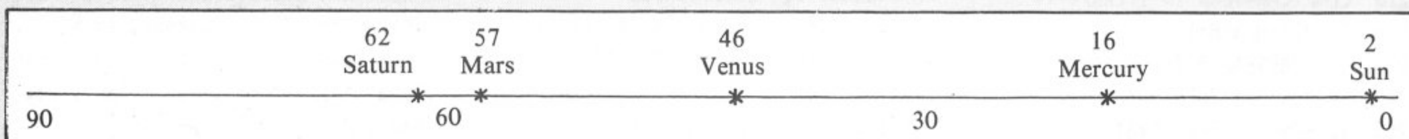
Figure II: Position of planets along the ecliptic at 6pm GMT, March 21 1972
