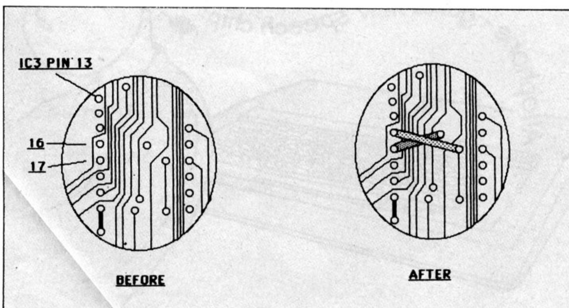
Figure II: IC3 pin 16 and 17 cross
