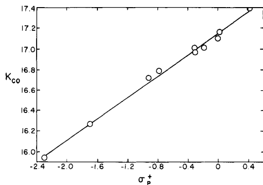
Figure 1. Correlation of carbonyl force constants with \sigma_p^+ for \text{Fp}(\eta\text{-CH}_2\text{=CRX}) cations.
