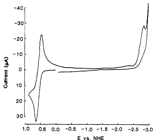
Figure 7. Cyclic voltammetry of 13 mM 11 in THF/0.2M TBAPF _6 ( v = 200 mV/s).
