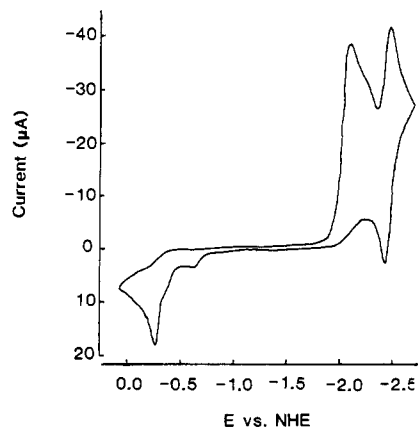
Figure 4. Cyclic voltammetry of 5.2 mM 6 in THF/0.2 M TBAPF 6 ( \nu = 200 \text{ mV/s} ).
