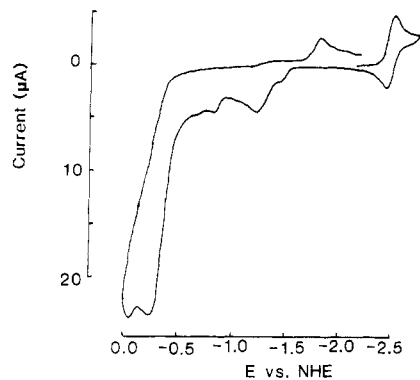
Figure 6. Cyclic voltammetry of the solution shown in Figure 5, after reduction at -2.60 V under CO atmosphere. Notice the new oxidation peak at -1.1 V, corresponding to 1 ( ML_x = W(CO)_3^- ; M'L_y = Fe(CO)_2^- ; v = 200 mV/s).
