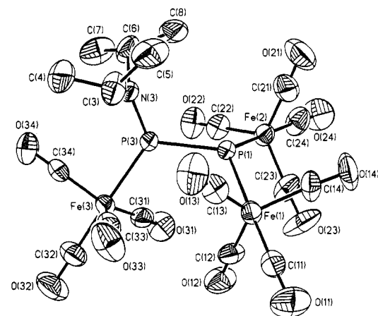
Figure 2. Structure of complex 10 showing the atomic numbering scheme with the ellipsoids at the 30% probability level.
