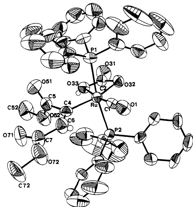
Figure 2. ORTEP 8 drawing of the molecular structure of [\text{Ru}(\text{CO})(\text{MeOCC}=\text{CHCOOMe})(\text{HCO}_3)(\text{PPh}_3)_2] ( 10 ) (atom numbering as in Table VI). Numbering of the carbons of the phenyl rings is omitted for clarity as are all the phenyl and methyl H atoms.
