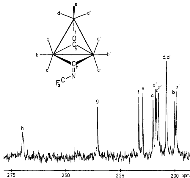
Figure 7. ^{13}\text{C} NMR spectra of \text{Fe}_3(\text{CO})_{11}(\mu_3\text{-CNCF}_3) at -100\text{ }^\circ\text{C} .
