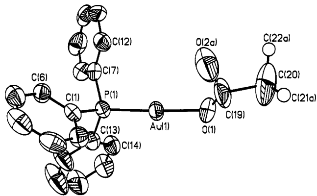
Figure 1. Structure of \text{Ph}_3\text{PAuO}_2\text{CCH}(\text{CH}_3)_2 (1). The thermal ellipsoids have been drawn at the 50% probability level.
