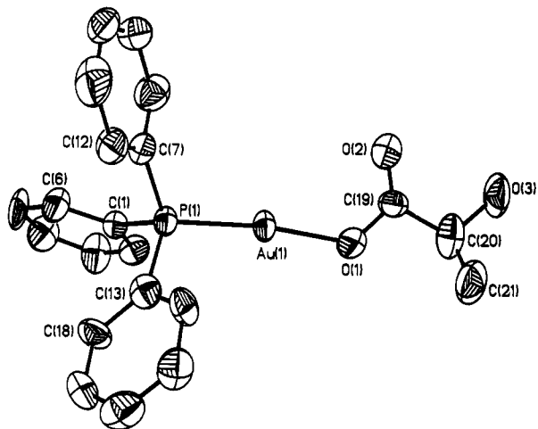
Figure 2. Structure of \text{Ph}_3\text{PAuO}_2\text{CCH}(\text{OH})\text{CH}_3 (2). The thermal ellipsoids have been drawn at the 50% probability level.
