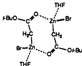
Figure 1. Schematic representation of the solid-state structure of a Reformatsky reagent, [\text{BrZnCH}_2\text{COO}(t\text{-Bu})\text{THF}]_2 .
