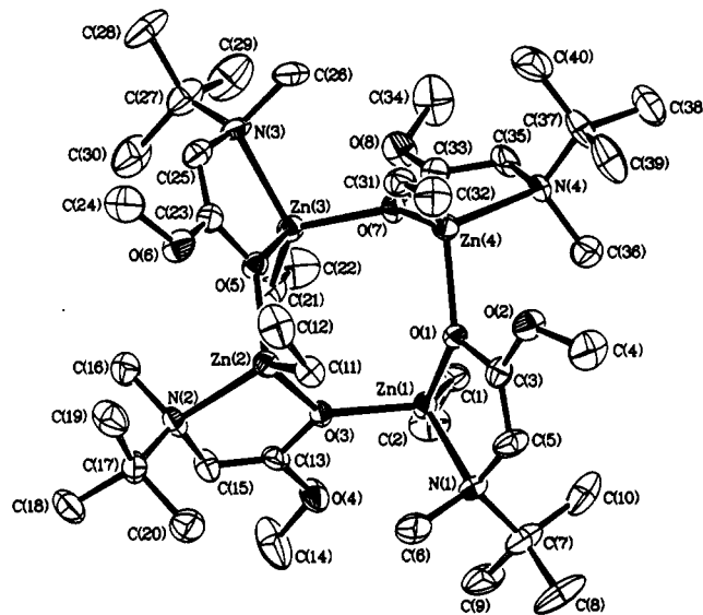
Figure 2. ORTEP drawing (30% probability level) of the molecular structure of [EtZnOC(OMe)=C(H)N( t -Bu)Me] 4 (4b), together with the adopted numbering scheme.
