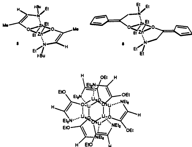
Figure 3. Schematic representations of the solid-state structures of some relevant enolates containing an intramolecular metal-nitrogen coordination.
