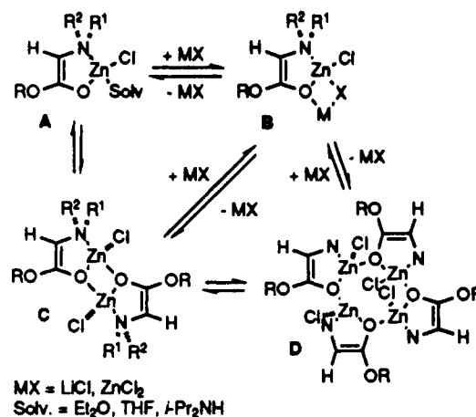
Figure 4. Schematic representations of the structures of chlorozinc enolate species, and equilibria between these species, that may be present in solutions.
