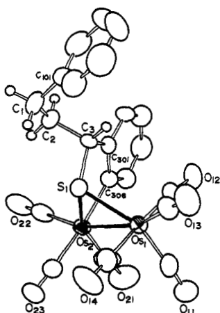
Figure 4. ORTEP diagram of \text{Os}_3(\text{CO})_7[\mu\text{-SC}(\text{H})(\text{C}_6\text{H}_4)\text{CH}_2\text{C}(\text{H})\text{Ph}] (3) showing 50% probability thermal ellipsoids.
