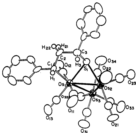
Figure 1. ORTEP diagram of \text{Os}_3(\text{CO})_{10}[\mu\text{-SC}(\text{H})\text{PhCH}_2\text{C}(\text{H})\text{Ph}] ( cis -1) showing 50% probability thermal ellipsoids.
