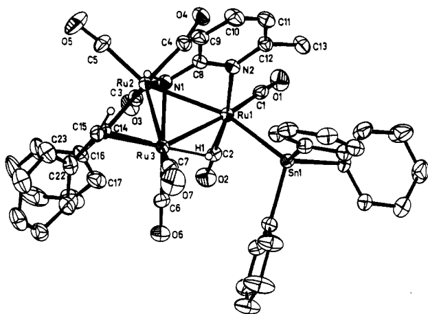
Figure 1. Molecular structure of [Ru 3 (μ-H)(μ 3 ,η 2 -ampy){μ,η 1 :η 2 -PhC=C(H)Ph}(SnPh 3 )(CO) 7 ] (isomer 5b) with thermal ellipsoids drawn at the 30% probability level.
