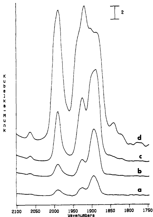
Figure 5. DRIFT spectra in the \nu(\text{CO}) region of [\text{Ni}(\text{NP}_2)] in a flow of CO at room temperature: (a) 10 min; (b) 20 min; (c) 30 min; (d) 90 min.
