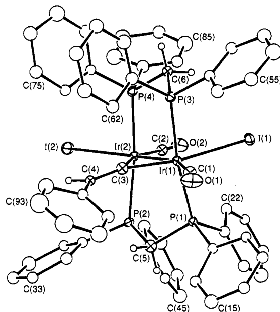
Figure 2. Perspective view of [\text{Ir}_2\text{I}_2(\text{CO})_2(\mu\text{-CC}(\text{H})\text{Ph})\text{-(dppm)}_2] (7). Thermal ellipsoids are shown at the 20% level, except for methylene and vinylidene hydrogens, which are shown arbitrarily small; phenyl hydrogens are omitted.
