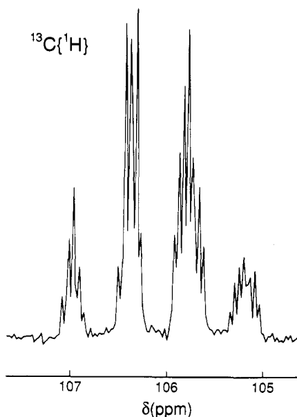
Figure 3. ^{13}\text{C}\{^1\text{H}\} NMR spectrum of complex 4 , showing the acetylenic region. ^{13}\text{C} -enriched acetylene was used in the preparation of 4 .
