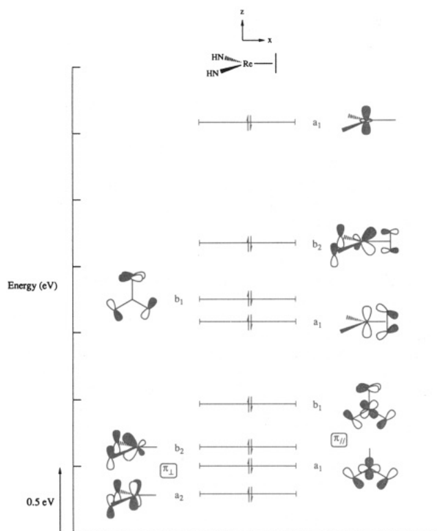
Figure 8. Orbital interaction diagram for [\text{Re}(\text{NH})_2(\text{C}_2\text{H}_2)]^- .
