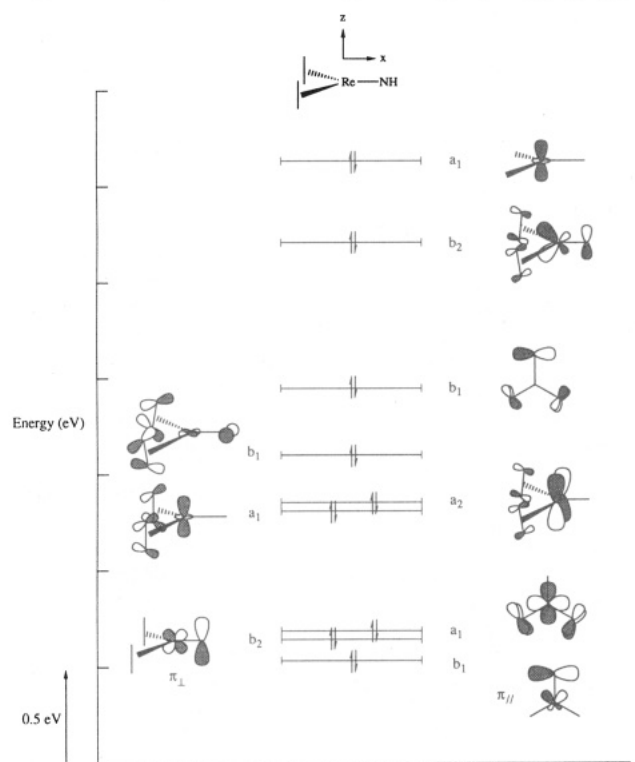
Figure 9. Orbital interaction diagram for [\text{Re}(\text{NH})(\text{C}_2\text{H}_2)_2]^- .
