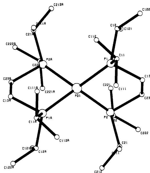
Figure 2. X-ray structure of 1d.
