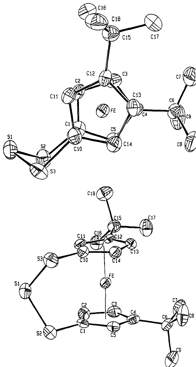
Figure 3. ORTEP drawing of the non-hydrogen atoms in (t\text{-Bu})_2\text{fcS}_3 .
