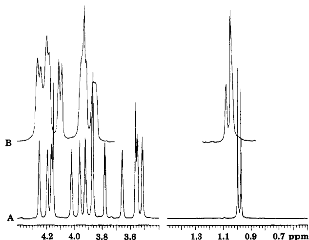
Figure 1. 400 MHz ^1\text{H} NMR spectra of \text{C}_6\text{D}_6 solutions of (A) t\text{-BuFcS}_3 and (B) [t\text{-BuFcS}_2]_n .
