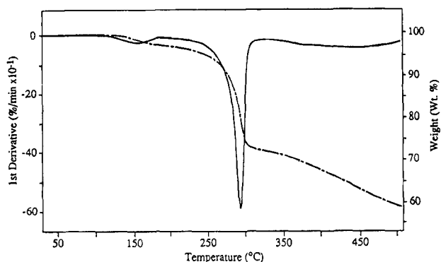
Figure 5. Thermogravimetric analysis of [t\text{-Bu}fcS_2]_n (heat rate of 10 °C/min, flowing He).
