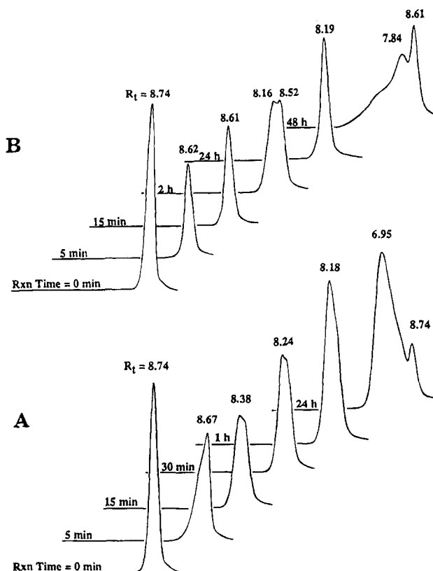
Figure 6. GPC traces for various stages in the desulfurization of (A) t\text{-Bu}fcS_3 and (B) (t\text{-Bu})_2fcS_3 with 0.95 equiv of Bu_3P (mobile phase CH_2Cl_2 , elution rate 1.5 mL/min, R_t = retention time).
