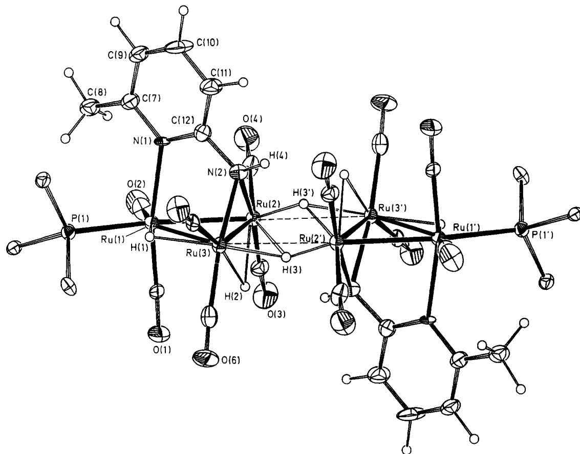
Figure 1. X-ray molecular structure of 3 . The primed atoms are related to the unprimed ones by an inversion center. For clarity, only the C_{\text{ortho}} atoms of the p -tolyl groups are shown.
