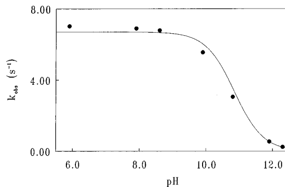
Figure 4. Plot of k_{\text{obs}} vs pH for the reaction of complex 1 with tmtu as entering nucleophile. Experimental conditions: [\text{Pt}] = 5 \times 10^{-5} M, T = 25 °C, [\text{I}^-] = 0.1 M ( \text{NaClO}_4 ), [\text{tmtu}] = 6 \times 10^{-4} M.
