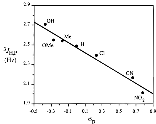
Figure 7. Plot of ^3J_{\text{H,P}} versus \sigma_p . For data see Table 2.
