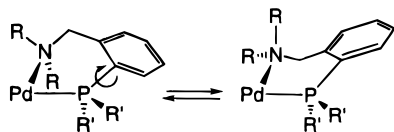
Figure 5. Conformational interconversion of the coordinated PCN ligand.
