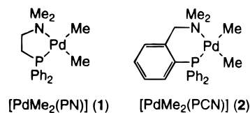
Figure 1. Schematic representation of the P,N-ligated complexes 1 and 2 .
