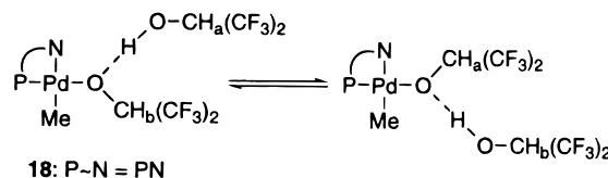
Figure 4. Intramolecular exchange of coordinated alkoxide and associated alcohol.
