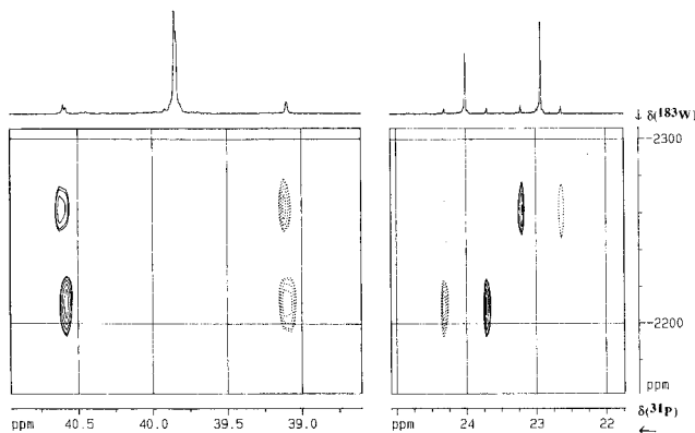
Figure 2. 161.98 MHz ^{31}\text{P} , ^{183}\text{W}\{^1\text{H}\} HMQC spectrum of a mixture of 2a and 2a' in a ratio of 40:60. The dephasing delay of ^1J(\text{P–W}) was set to 2.9 ms, and 112 t_1 increments were recorded with an accumulation of 128 scans each. The spectrum was acquired in the TPPI mode without refocusing. Negative cross peaks are represented by dotted lines. All other parameters were as described in the Experimental Section.
