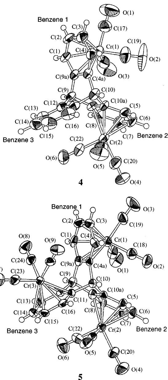
Figure 1. ORTEP drawings of 4 and 5 with thermal ellipsoids at 50% probability (solvent molecules are not shown).
