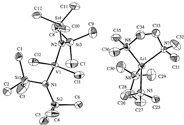
Figure 3. ORTEP drawing (50% ellipsoids) of one of the crystallographically independent molecules of \{[\text{Li}(\text{TMEDA})_2]\} \{[(\text{Me}_3\text{Si})_2\text{N}]_2\text{VCl}_2\} .
