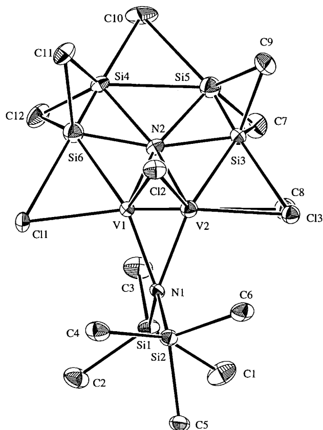
Figure 1. ORTEP drawing (50% ellipsoids) of [(Me 3 Si) 2 N] 2 VCl 2 . V(2), Si(5), Si(6), and Cl(3) are at 16% occupancy, while V(1), Si(3), Si(4), and C(8) are at 84% occupancy. The position of the (minor occupancy) carbon atom near Cl(1) was not resolved.
