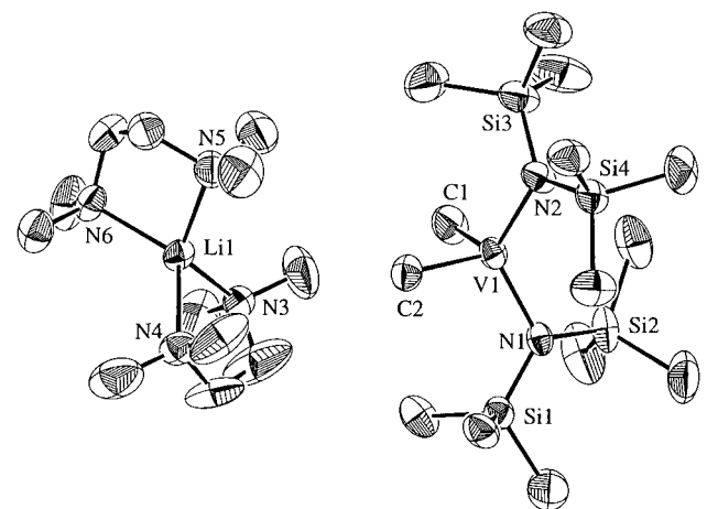
Figure 4. ORTEP drawing (50% ellipsoids) of one of the crystallographically independent molecules of [\text{Li}(\text{TMEDA})_2]\{[(\text{Me}_3\text{Si})_2\text{N}]_2\text{VMe}_2\} .
