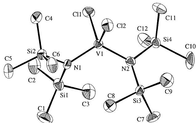
Figure 2. ORTEP drawing (50% ellipsoids) of the major conformer of [(\text{Me}_3\text{Si})_2\text{N}]_2\text{VCl}_2 .
