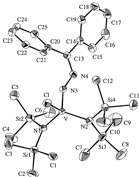
Figure 5. ORTEP drawing (50% ellipsoids) of [(\text{Me}_3\text{Si})_2\text{N}]_2\text{V}(\text{Cl})(\text{N}_2\text{CPh}_2) .
