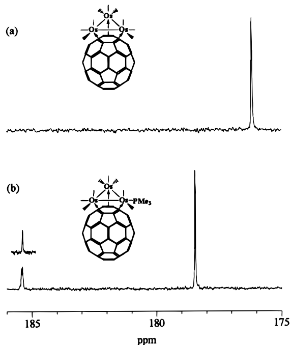
Figure 4. (a) 13 C NMR spectrum (151 MHz, CO region, 298 K, \text{CS}_2/\text{ext.CD}_2\text{Cl}_2 ) of 6* . (b) 13 C NMR spectrum (151 MHz, CO region, \text{CS}_2/\text{C}_6\text{D}_6 ) of 7* . The inset is from the 13 C{ 31 P} NMR spectrum.
