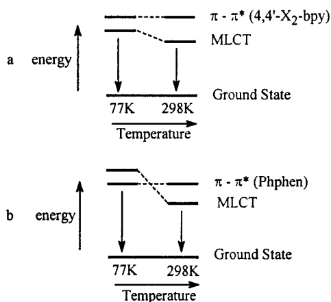
Figure 7. State diagram for the lowest triplet states of (a) [\text{HNCH}_2\text{CH}_2\text{NHCr}(\text{4,4}'\text{-X}_2\text{-bpy})(\text{CO})_3]^+ ( 2–6 ) and (b) [\text{HNCH}_2\text{CH}_2\text{NHCr}(\text{Phphen})(\text{CO})_3]^+ ( 7 ).
