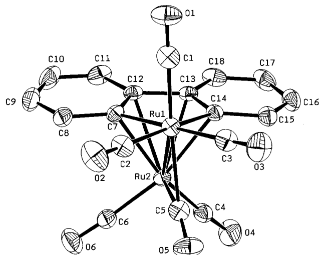
Figure 2. Molecular structure of Ru 2 (CO) 5 (μ-CO)(μ-η 2 ,η 4 -(C 6 H 4 ) 2 ) ( 2 ). The hydrogen atoms have been artificially omitted for clarity.
