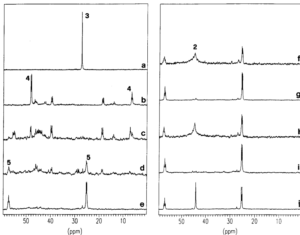
Figure 3. ^{31}\text{P}\{^1\text{H}\} NMR study (sapphire tube, \text{THF}-d_6 , 81.01 MHz) of the catalytic hydrogenolysis of BT in the presence of 3 (30 bar of \text{H}_2 , substrate/catalyst ratio 30, substrate/ \text{KOBU}^t ratio 10): (a) pure sample of 3 ; (b) at 20 °C for 30 min; (c) at 40 °C for 30 min; (d) at 40 °C for 1.5 h; (e) at 40 °C for 3 h; (f) at 70 °C for 30 min; (g) after the tube was cooled to 40 °C; (h) after the tube was heated to 70 °C for 30 min; (i) after 1 day at 20 °C.
