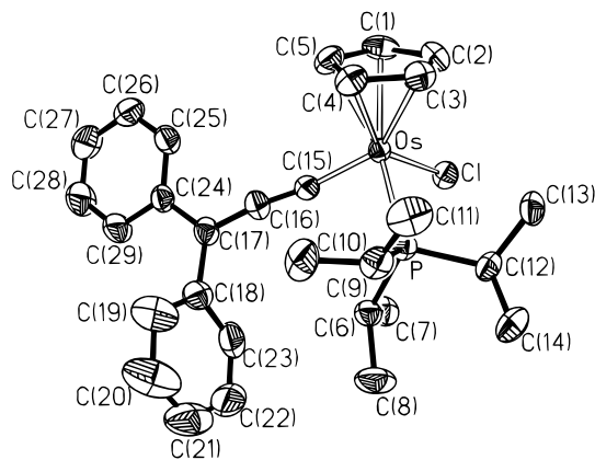
Figure 1. Molecular diagram of the complex \text{Os}(\eta^5\text{-C}_5\text{H}_5)\text{Cl}(\text{=C=C=CPh}_2)(\text{P}^i\text{Pr}_3) ( 3 ). Thermal ellipsoids are shown at 50% probability.
