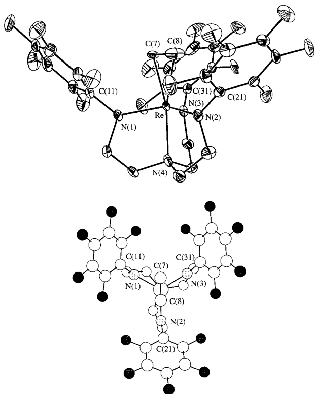
Figure 3. (a) Side view (ORTEP) of the structure of [\text{N}_3\text{NF}]\text{Re}(\text{C}_2\text{H}_4) . (b) Top view of the structure of [\text{N}_3\text{NF}]\text{Re}(\text{C}_2\text{H}_4) .
