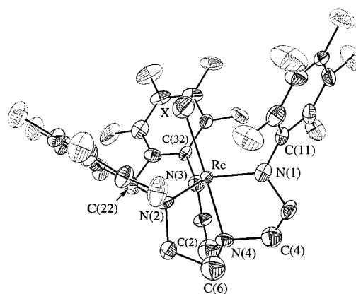
Figure 2. Side view (ORTEP) of the structure of [\text{N}_3\text{N}_F]\text{ReX} , where X = 0.60Br/0.40Cl.
