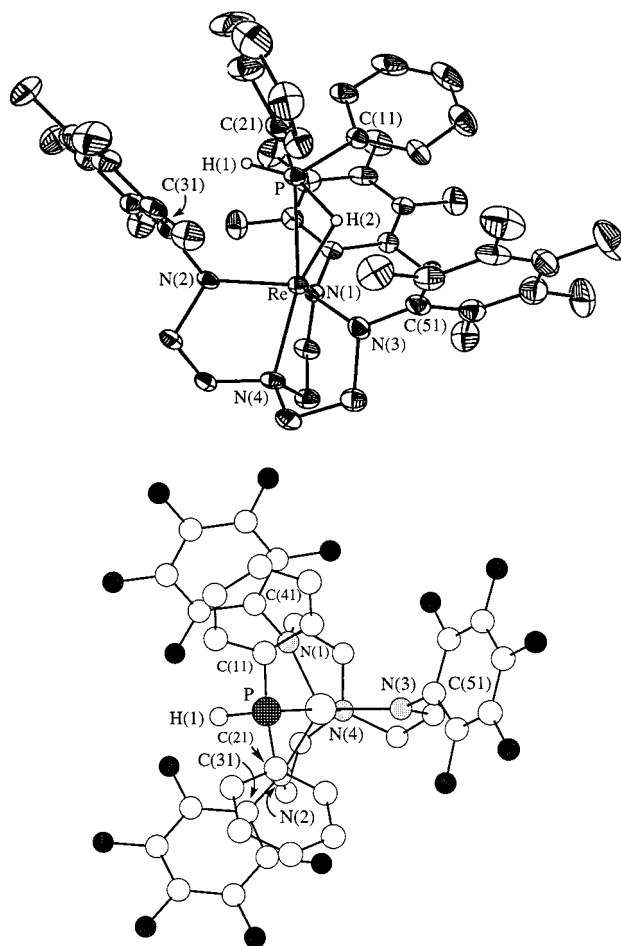
Figure 5. (a) Side view (ORTEP) of the structure of \{[\text{N}_3\text{N}_F]\text{Re}(\text{PPh}_2\text{H})(\text{H})\}^+ . (b) Top view of the structure of \{[\text{N}_3\text{N}_F]\text{Re}(\text{PPh}_2\text{H})(\text{H})\}^+ (H(2) left out for clarity).
