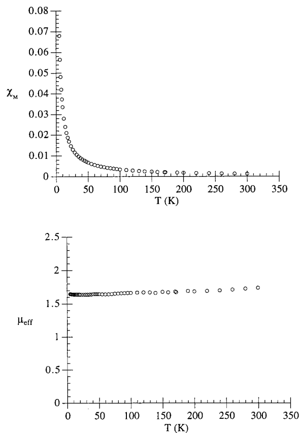
Figure 1. Plots of \chi_M (top) and \mu_{\text{eff}} (bottom) vs T for [\text{N}_3\text{N}_\text{F}]\text{-ReBr} .
