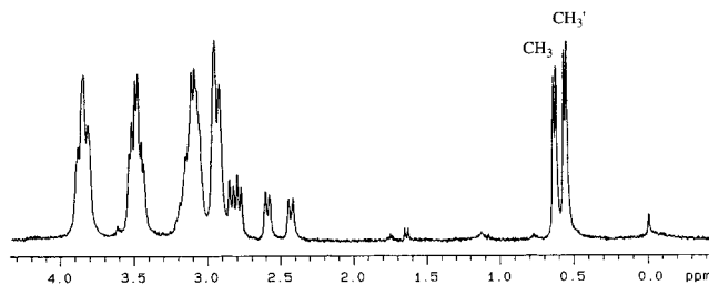
Figure 4. ^1\text{H} NMR spectrum ( \text{CD}_2\text{Cl}_2 , -90^\circ\text{C} ) of [\text{N}_3\text{NF}]\text{Re}(\text{CH}_3\text{CH}=\text{CH}_2) .
