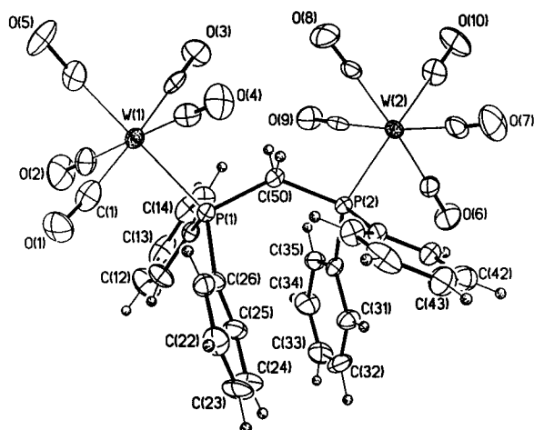
Figure 3. Molecular structure of (OC)_5W(\mu\text{-dppm})W(CO)_5 (2).
