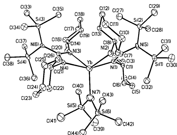
Figure 2. ORTEP diagram for 8 . Thermal ellipsoids are drawn at 30% probability. Selected bond distances (Å) and angles (deg): Yb–N(1) 2.329(13), Yb–N(2) 2.301(15), Yb–N(3) 2.311(13), Yb–N(4) 2.328(12), Yb–N(7) 2.343(19), N(1)–Yb–N(2) 58.0(5), N(3)–Yb–N(4) 57.9(4), N(1)–Yb–N(7) 100.6(6), N(2)–Yb–N(7) 119.4(6), N(3)–Yb–N(7) 124.6(6), N(4)–Yb–N(7) 104.6(6), C(7)–N(1)–Yb 94.5(10), C(7)–N(2)–Yb 93.7(11), C(7)–N(5)–Si(1) 118.7(11), C(7)–N(5)–Si(2) 118.5(11), Si(1)–N(5)–Si(2) 122.7(8), C(20)–N(3)–Yb 92.7(10), C(20)–N(3)–Yb 92.7(10).
