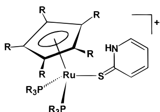
R = H; \text{PR}_3 = \text{PEt}_3 8 R = H; \text{PR}_3 = \text{PPh}_3, \text{PMe}^i\text{Pr}_2 9 R = Me; \text{PR}_3 = \text{PEt}_3 10
