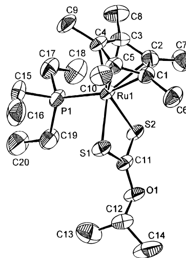
Figure 2. ORTEP drawing (50% probability thermal ellipsoids) of [\text{Cp}^*\text{Ru}(\text{S}_2\text{CO}^i\text{Pr})(\text{PEt}_3)] . H atoms are omitted.
