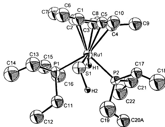
Figure 1. ORTEP drawing of the cation [\text{Cp}^*\text{RuH}(\text{SH})(\text{PET}_3)_2]^+ with 50% probability thermal ellipsoids. H atoms, except hydride and that on the mercapto ligand, are omitted.
