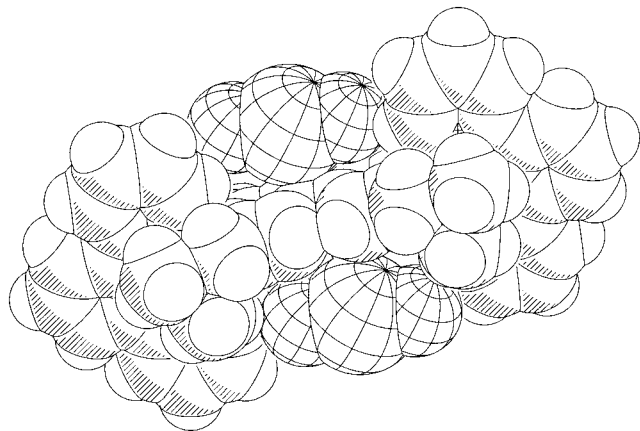
Figure 5. PLUTON space-filling structure of the complex tetracation [(\text{Ru}^{\text{III}})_2(4,4'\text{-}\{\text{C}_6\text{H}_2(\text{CH}_2\text{NMe}_2)_2\text{-}2,6\}_2)(\text{terpy})_2]^{4+} of 5a , together with two of the \text{CuCl}_2^- anions that pack above and below the biphenylene bridge.
