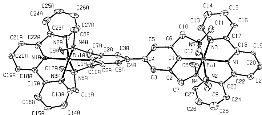
Figure 3. ORTEP drawing (50% probability atomic displacement ellipsoids) of the complex dication [(Ru^{II})_2(4,4'\text{-}\{C_6H_2(CH_2-NMe_2)_2-2,6\}_2)(terpy)_2]^{2+} of 8 . Hydrogen atoms, cocrystallized solvent molecules, and PF_6^- counterions have been omitted for clarity. Selected bond distances in angstroms (esds in parentheses): Ru(1)–C(1), 2.003(16)/2.002(16); Ru(1)–N(1), 2.003(16)/2.002(14); Ru(1)–N(2), 2.085(16)/2.089(15); Ru(1)–N(3), 2.094(15)/2.092(15); Ru(1)–N(4), 2.176(13)/2.171(13); Ru(1)–N(5), 2.164(13)/2.156(13); C(4)–C(4)A, 1.47(3); Ru(1)⋯Ru(1)A, 11.066(3). Selected bond angles in degrees (esds in parentheses): C(1)–Ru(1)–N(4), 78.3(6)/79.2(6); C(1)–Ru(1)–N(5), 77.9(7)/77.5(6); N(4)–Ru(1)–N(5), 156.1(6)/156.6(6).
