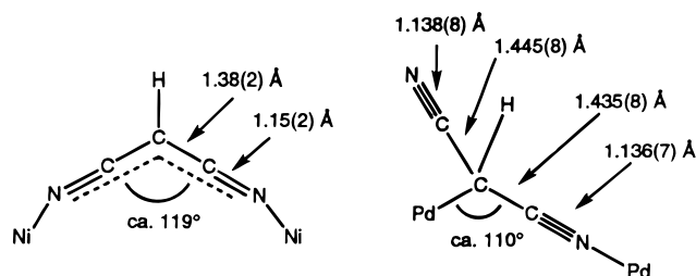
Figure 4. Relevant structural parameters for N,N - and C,N -bonded dicyanomethanide.
