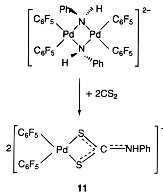
Scheme 3
