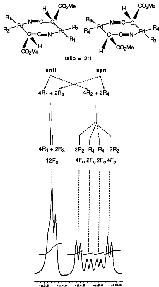
Figure 2. ^{19}F NMR spectrum of complex 13 in the o -fluorine region.
