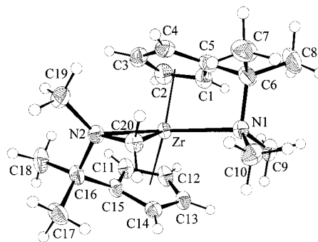
Figure 4. Molecular structure of 8 (cation only, with unsystematic atom-numbering scheme). Selected bond lengths (Å) and angle (deg): Zr–N1 = 2.4692(12), Zr–N2 = 2.2930(12), Zr–C20 = 2.2510(14), N1–C6 = 1.552(2), C6–C5 = 1.515(2), C20–N2 = 1.4640(18), N2–C16 = 1.514(2), C16–C15 = 1.516(2); N1–Zr–N2 = 123.61(4), N1–Zr–C20 = 86.43(5), N2–Zr–C20 = 37.58(5), Zr–N1–C6 = 97.36(8), N1–C6–C5 = 101.57(12), Zr–N2–C20 = 69.66(7), Zr–N2–C16 = 102.10(8), Zr–C20–N2 = 72.77(7), C20–N2–C16 = 116.78(12), N2–C16–C15 = 101.14(11).
