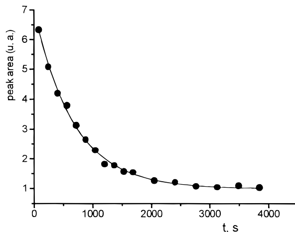
Figure 1. Peak area, as a function of time, of the 1 H NMR signal of coordinated CH 3 CN after addition of CD 3 CN (8.1 μL, 30.81 mM) to a solution of [RuCp(PMe 3 )(CH 3 CN) 2 ] + ( 2b ; 25 mM) in CD 3 NO 2 at 295 K.
