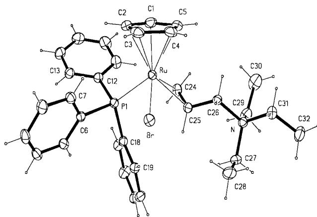
Figure 5. Structural view of [\text{RuCp}(\eta^2\text{-CH}_2=\text{CHCH}_2\text{NEt}_3)(\text{PPh}_3)\text{Br}]\text{PF}_6\cdot\text{CH}_2\text{Cl}_2 ( 9 · \text{CH}_2\text{Cl}_2 ) showing 20% thermal ellipsoids ( \text{PF}_6^- and \text{CH}_2\text{Cl}_2 omitted for clarity). Selected bond lengths (Å) and angles (deg): Ru(1)–C(1–5) av = 2.216(3), Ru–P(1) = 2.315(1), Ru–Br = 2.565(1), Ru–C(24) = 2.172(3), Ru–C(25) = 2.193(3), C(1)–C(2) = 1.403(5), C(2)–C(3) = 1.380(6), C(3)–C(4) = 1.425(5), C(4)–C(5) = 1.385(5), C(1)–C(5) = 1.403(5), C(24)–C(25) = 1.392(4); C(24)–Ru–C(25) = 37.2(1), C(24)–Ru–P(1) = 98.5(1), C(25)–Ru–P(1) = 85.2(1).
