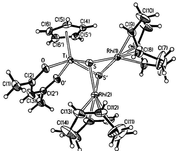
Figure 2. Molecular structure of [\text{Cp}(\text{acac})\text{Ti}(\mu_3\text{-S})_2\{\text{Rh}(\text{cod})\}_2] ( 1 ) showing the atom-numbering scheme used (symmetry transformation for primed atoms: x, 1/2-y, z ).
