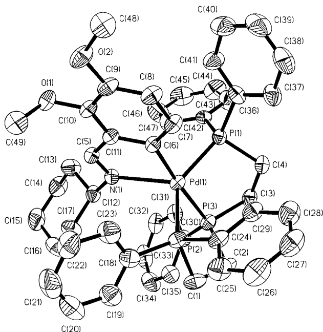
Figure 2. Structure of the cation for compound 2 showing the atom-numbering scheme. Hydrogen atoms were omitted for clarity.
