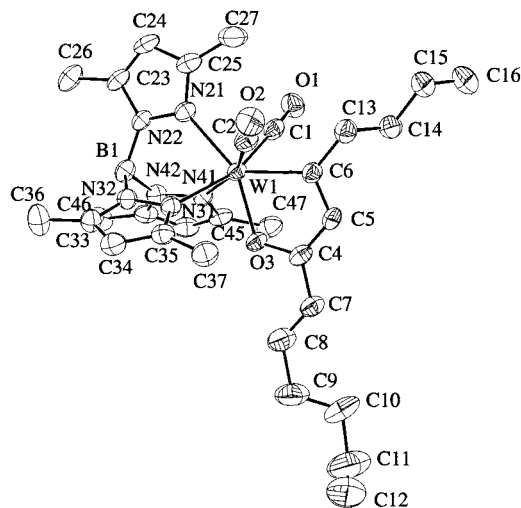
Figure 3. ORTEP representation of \text{Tp}'(\text{CO})_2\text{W}(\eta^2(\text{C},\text{O})\text{-C}(\text{Bu}^n)\text{CHC(=O)CH=CHBu}^n) ( 12 ).
