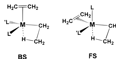
Scheme 4. Backside and Frontside Olefin Complex
