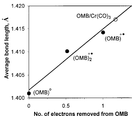
Figure 4. Linear increase in the average (aromatic) bond lengths in OMB attendant upon the successive removal of 0.5 and 1.0 electron in (OMB) 2 •+ and OMB •+ , respectively. The fit of the point for the (OMB)Cr(CO) 3 complex indicates an effective degree of charge (electron) transfer of essentially unity.
