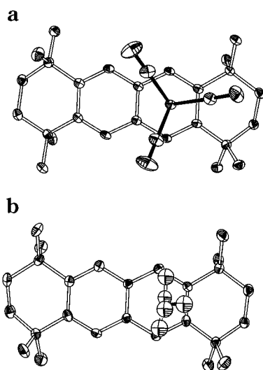
Figure 7. Complexation of the naphthalenoid donor OMN with \text{Cr}(\text{CO})_3 (a) and \text{NO}^+ (b) showing the preferential complexation with a single (benzenoid) ring reminiscent of that shown for the biphenylene donor in Figure 6.
