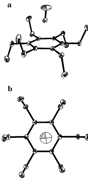
Figure 9. Axial bonding of \text{NO}^+ along the 3-fold symmetry axis of the sterically encumbered HEB donor in side (45°) and top perspectives (a and b, respectively), showing the equivalence of all aromatic C–C bonds in contrast to those in the [ HMB , \text{NO}^+ ] complex in Figure 2.
