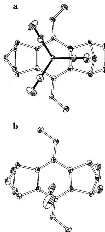
Figure 5. Rotation of the pair of methoxy groups in CRET (top perspective) upon its complexation with Cr(CO) 3 (a) and NO + (b). Compare with the conformational change of the methoxy groups in CRET •+ relative to CRET in Figure 3.
