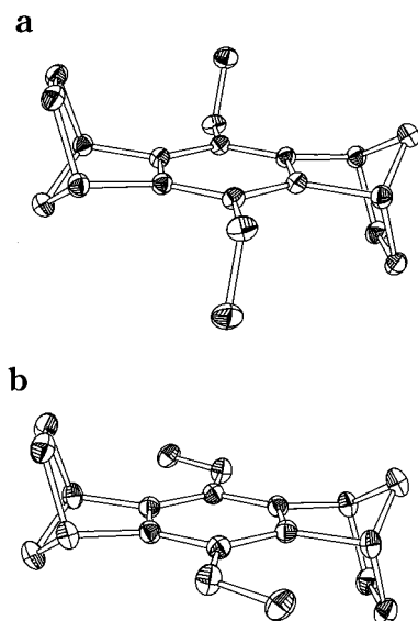
Figure 3. Aromatic donor CRET (a) and its cation radical CRET •+ (b) showing the 90° rotation of both methoxy groups upon one-electron oxidation.
