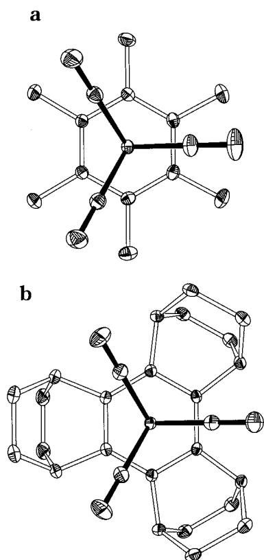
Figure 1. Molecular structures (top perspective) of typical (arene)Cr(CO) 3 complexes where arene = HMB (a) and TET (b) as described in Chart 1. Hydrogens are omitted for clarity. Thermal ellipsoids are shown at 50% probability level.
