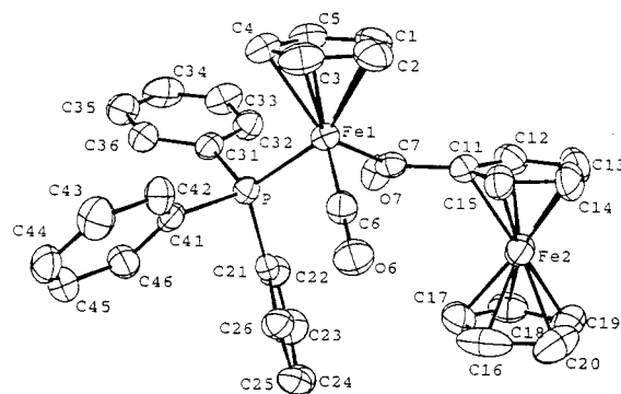
Figure 2. Molecular plot of (\eta^5\text{-C}_5\text{H}_5)\text{Fe}[\mu,\eta^5:\text{C-C}_5\text{H}_4\text{C}(\text{O})]\text{Fe}(\text{CO})(\text{PPh}_3)(\eta^5\text{-C}_5\text{H}_5) ( 2 ) with the atomic numbering sequence. The thermal ellipsoids are drawn at the 50% probability level with H atoms omitted for clarity. Selected bond lengths (Å): Fe1–P 2.202(2), Fe1–C1 2.121(5), Fe1–C2 2.111(5), Fe1–C3 2.126(6), Fe1–C4 2.132(5), Fe1–C5 2.114(5), Fe1–C6 1.722(5), Fe1–C7 1.963(5), C6–O6 1.160(7), C7–O7 1.223(6), C7–C11 1.509(7), P–C21 1.834(5), P–C31 1.848(5), P–C41 1.846(5). Selected bond angles (deg): P–Fe1–C6 91.1(2), P–Fe1–C7 93.4(2), C6–Fe1–C7 92.0(2), Fe1–C6–O6 178.1(5), Fe1–C7–O7 119.5(4), C7–C11–Fe2 124.7(4).
