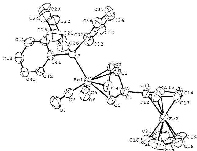
Figure 1. Molecular plot of (\eta^5\text{-C}_5\text{H}_5)\text{Fe}[\mu,\eta^5:\eta^4\text{-5-}exo\text{-}(1'\text{-C}_5\text{H}_4)\text{C}_5\text{H}_5]\text{Fe}(\text{CO})_2(\text{PPh}_3) ( 1 ) with the atomic numbering sequence. The thermal ellipsoids are drawn at the 50% probability level with H atoms omitted for clarity. Selected bond lengths (Å): Fe1–P 2.225(3), Fe1–C2 2.126(9), Fe1–C3 2.043(9), Fe1–C4 2.044(9), Fe1–C5 2.095(9), Fe1–C6 1.744(11), Fe1–C7 1.751(11), C6–O6 1.145(13), C7–O7 1.163(14), C1–C11 1.515(13), P–C21 1.848(10), P–C31 1.827(10), P–C41 1.845(9). Selected bond angles (deg): P–Fe1–C6 97.3(3), P–Fe1–C7 94.8(3), C6–Fe1–C7 102.2(5), Fe1–C6–O6 178.1(5), Fe1–C7–C11 119.5(4), C7–C11–Fe2 124.7(4).
