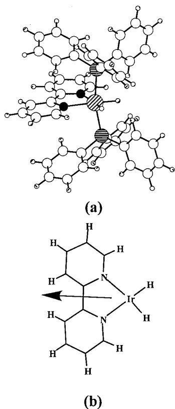
Figure 5. (a) Optimized geometry (ONIOM) for \text{Ir}(\text{H})_2\text{-(bipy)(PPh}_3)_2^+ . (b) Schematic representation of the QM part in the ONIOM calculations ( \text{PH}_3 groups have been omitted for clarity) showing the orientation of the dipole moment of the molecule.
