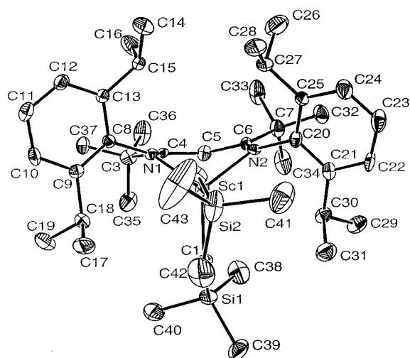
Figure 7. ORTEP diagram of the four-coordinate complex 6b (30% ellipsoids).
