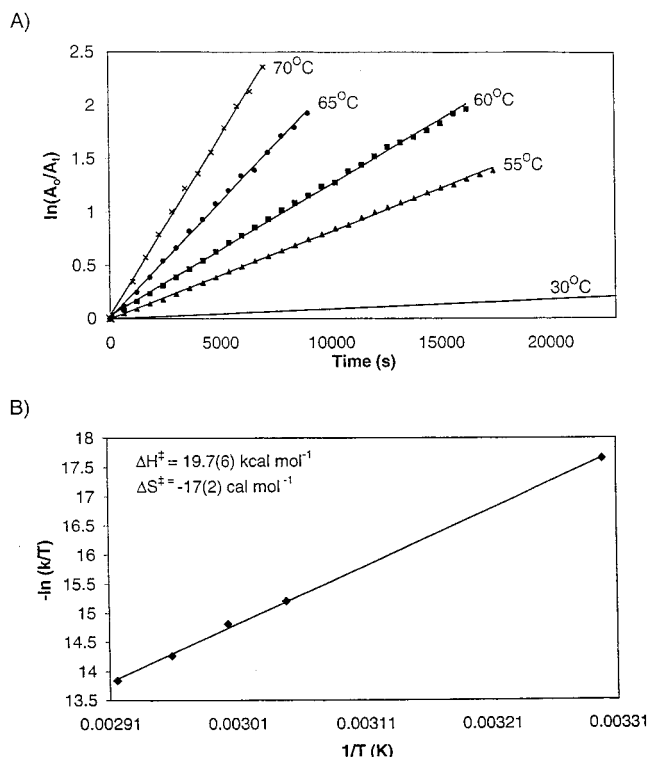
Figure 9. (A) First-order kinetic plots for the metalation of 6b to produce 13b and \text{SiMe}_4 at various temperatures. The complete data set for the run at 30^\circ\text{C} is not shown in the figure; this run took over 80 000 s to go to 5 half-lives. (B) Eyring plot of the temperature dependence of the rate constants.
