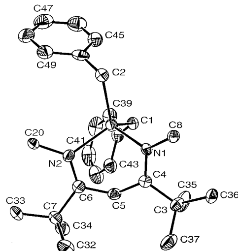
Figure 5. ORTEP diagram of the four-coordinate complex 4b (30% ellipsoids). Only the ipso carbons of the N aryl groups are shown for clarity.
