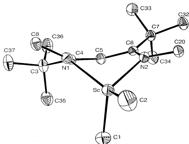
Figure 3. ORTEP diagram of the four-coordinate complex 2b (30% ellipsoids). Only the ipso carbons of the N aryl groups are shown for clarity.
