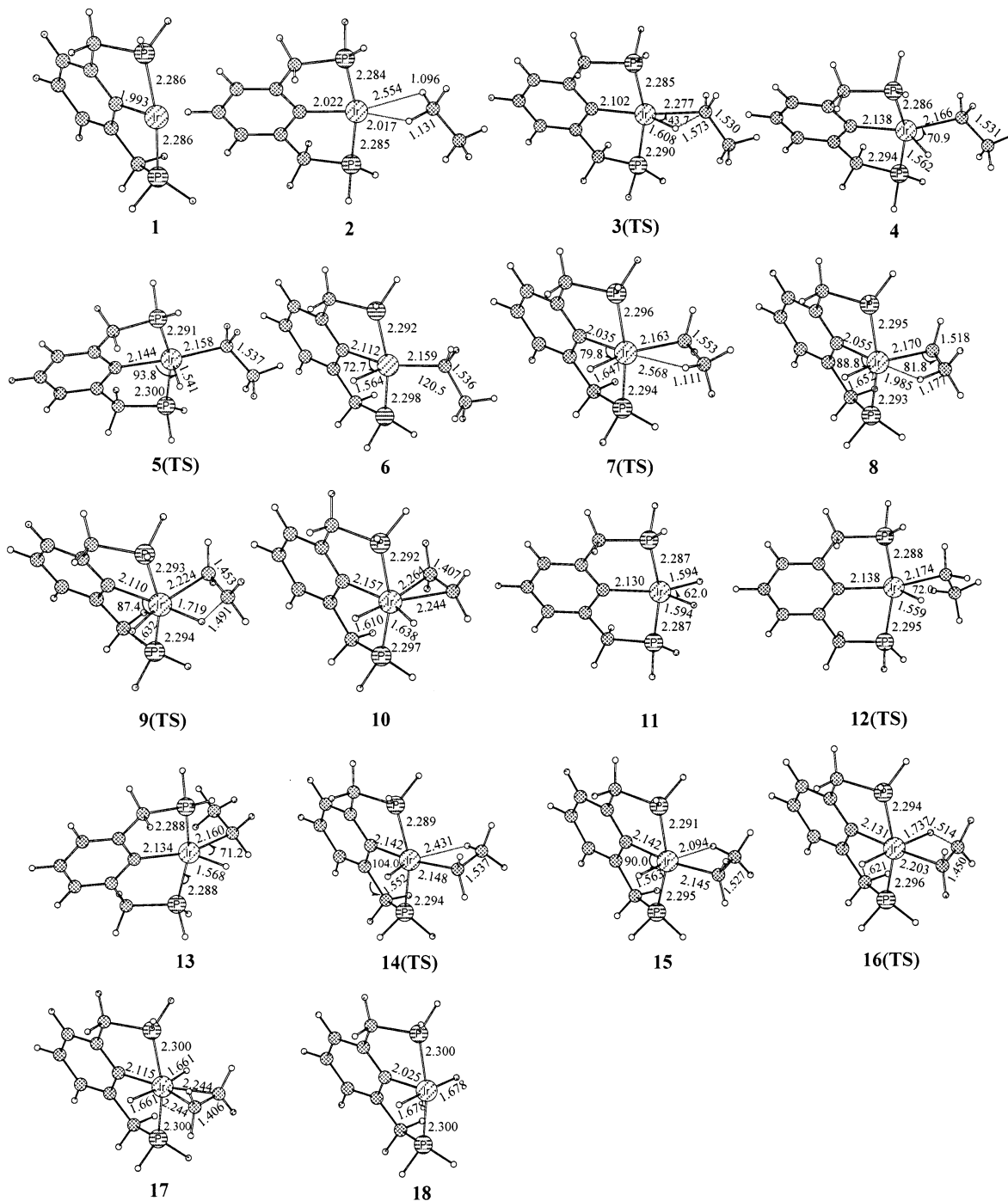
Figure 2. B3LYP-optimized structures of the reactant, intermediates, transition states, and products along the two pathways in Figure 1.
