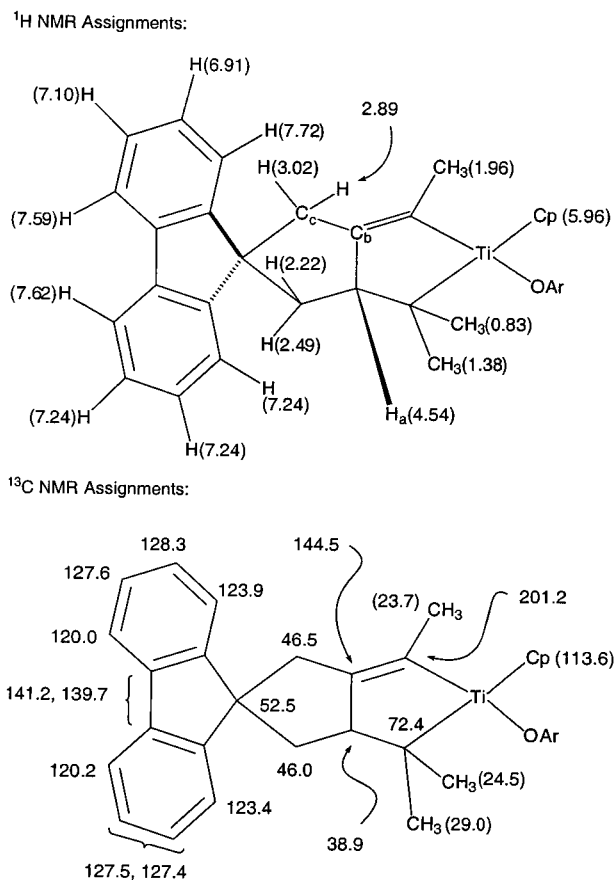
Figure 6. ^1H and ^{13}C assignments for metallacycle 9 .
