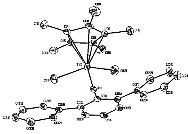
Figure 4. ORTEP plot of the solid-state molecular structure of 4a . Thermal ellipsoids are shown at the 30% probability level.
