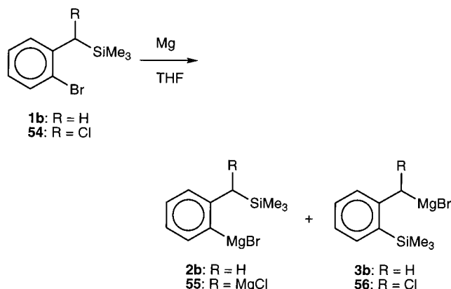
Scheme 15
