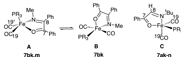
Figure 2. Three different geometries of complexes 7 .
