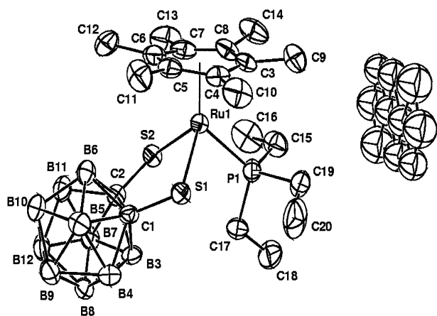
Figure 3. Molecular structure of 4b with atom labeling; ellipsoids show 30% probability levels and hydrogen atoms have been omitted for clarity.
