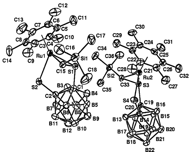
Figure 6. Molecular structure of 11b with atom labeling; ellipsoids show 30% probability levels and hydrogen atoms have been omitted for clarity.
