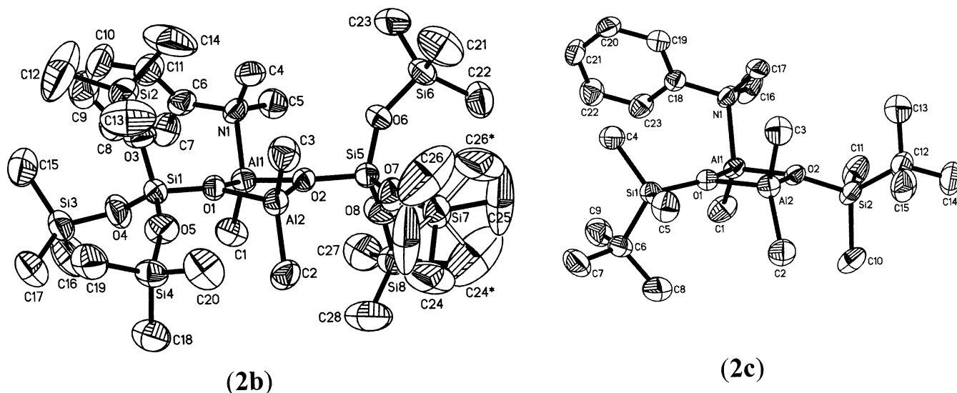
Figure 1. Structure of complexes 2b,c ( \text{B}(\text{C}_6\text{F}_5)_4^- anions omitted for clarity).
