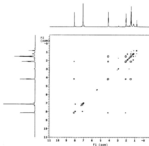
Figure 1. COSY spectrum of poly(pyrroline).
