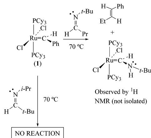
Scheme 3. Complex 1 Reacts with N - t -Bu Imine but Does Not React with Imines That Possess a t -Bu Group at the Imine Carbon
