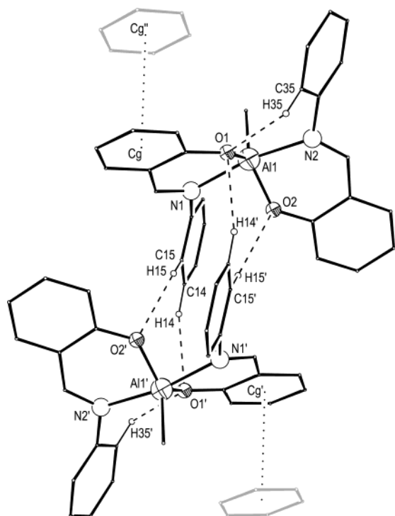
Figure 6. Hydrogen-bonded dimer of \text{MeAl}(\text{saldPh})_2 ( 4 ) in the solid state. The dashed lines represent intra- and intermolecular \text{C}-\text{H}\cdots\text{O} hydrogen bonds. The atoms labeled with a prime (') are at symmetry-equivalent positions ( 1-x, 1-y, -z ). Hydrogen atoms are omitted, excluding those involved in H-bond formation.
